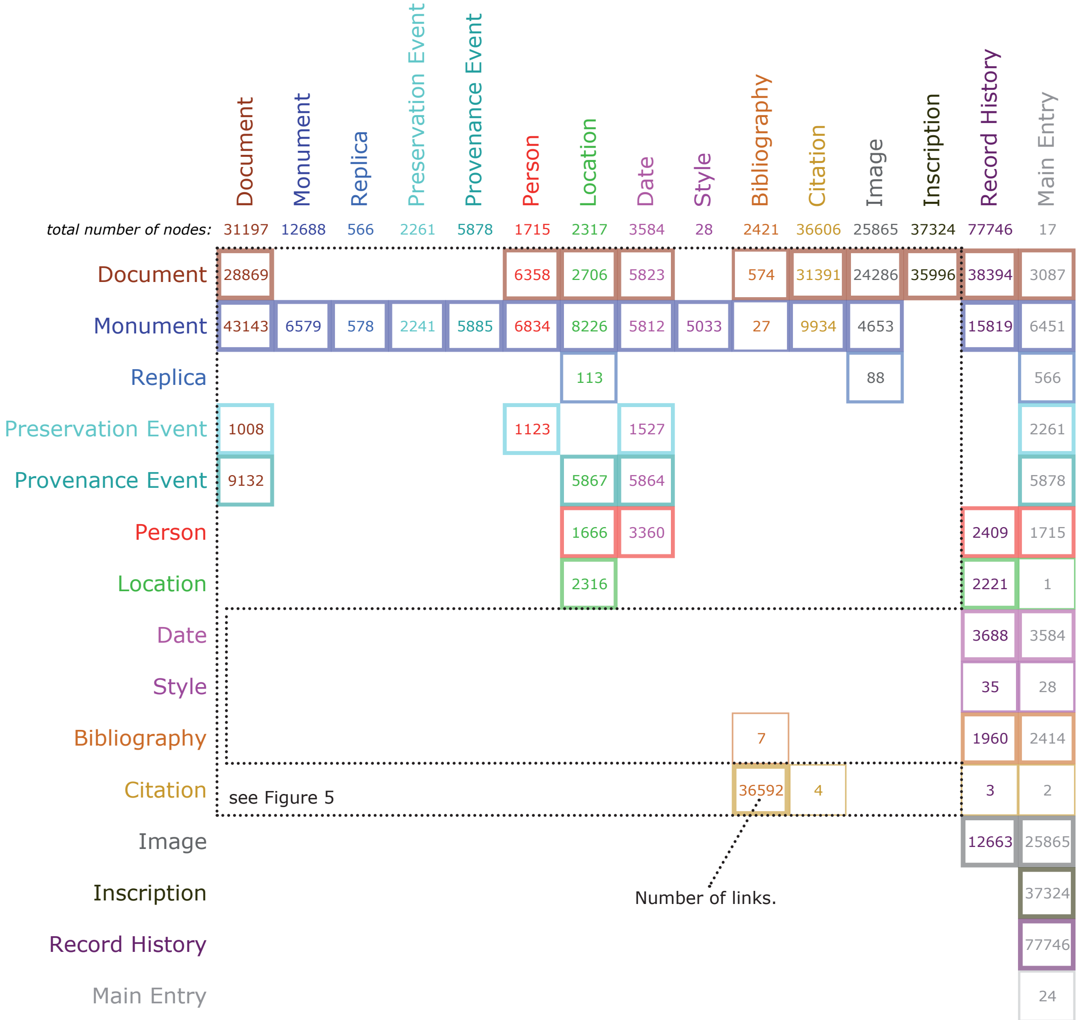
The CENSUS data model as a weighted adjacency matrix
